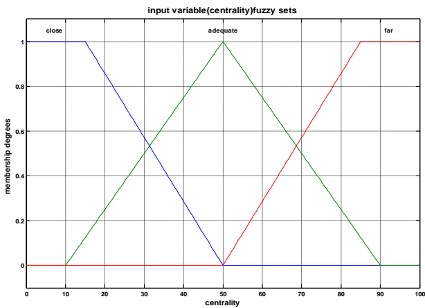
Fig. 6. Fuzzy set applied for variable centrality.
