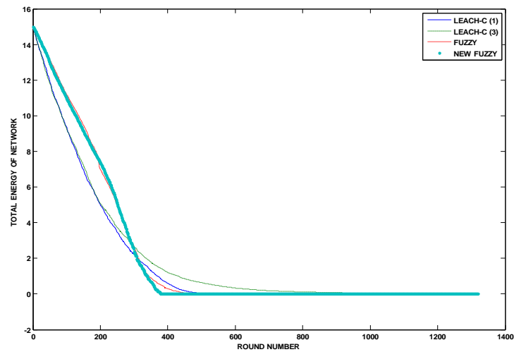
Fig. 10. Total energy available in the network by applying different cluster-head election algorithms with fixed nodes.
