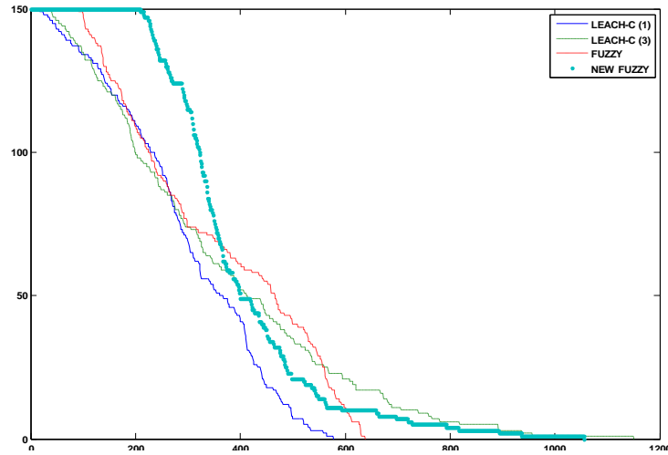
Fig. 9. Compression of network life time by applying different cluster-head election algorithms with mobile nodes.
