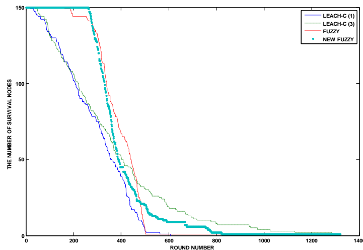
Fig. 8.compression of network life time by applying different cluster-head election algorithms with fixed nodes.
