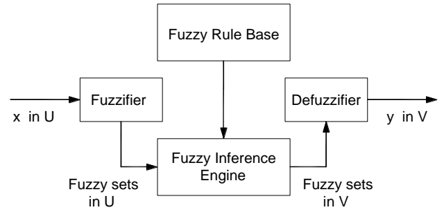
Fig. 3. Fuzzy system.
