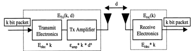
Fig. 2. Energy Consumption Model [3].
