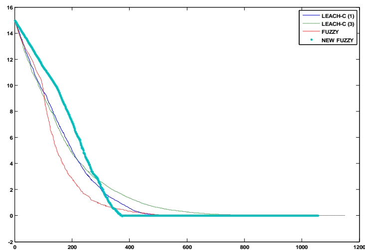
Fig. 11. Total energy available in the network by applying different cluster-head election algorithms with mobile nodes.
