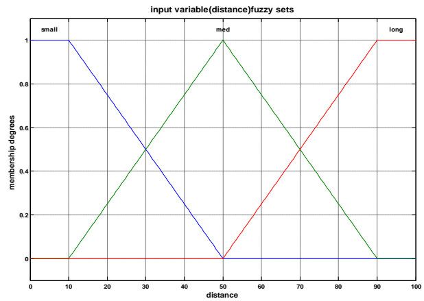
Fig.7. Fuzzy set applied for variable distance to the base station.
