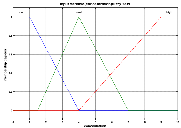
Fig. 5. Fuzzy set applied for variable concentration.
