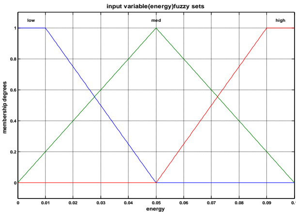
Fig. 4. Fuzzy set applied for variable energy.
