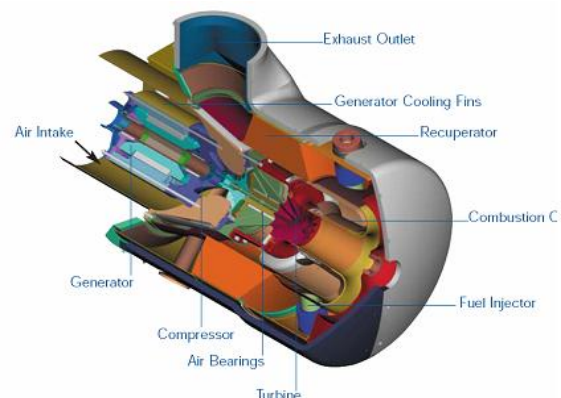
Fig.1 View of a Capstone microturbine [3]
