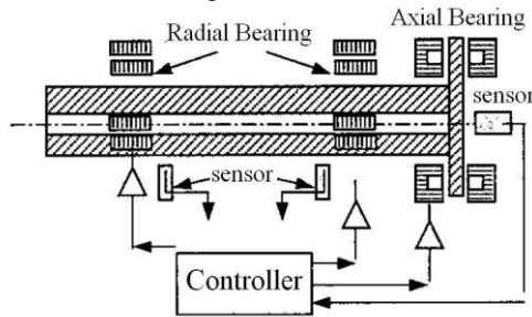
Fig. 7 Magnetic bearing
