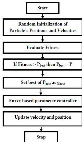
Fig. 1. Fuzzy Particle Swarm Optimization Diagram
