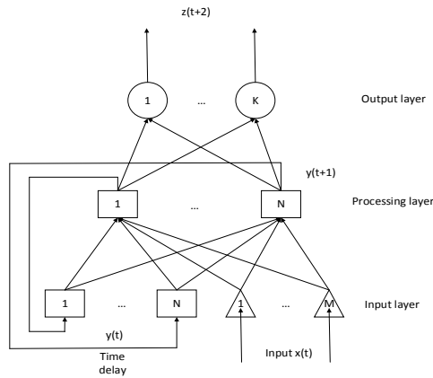
Fig. 2. RTRL for two-step-ahead prediction
